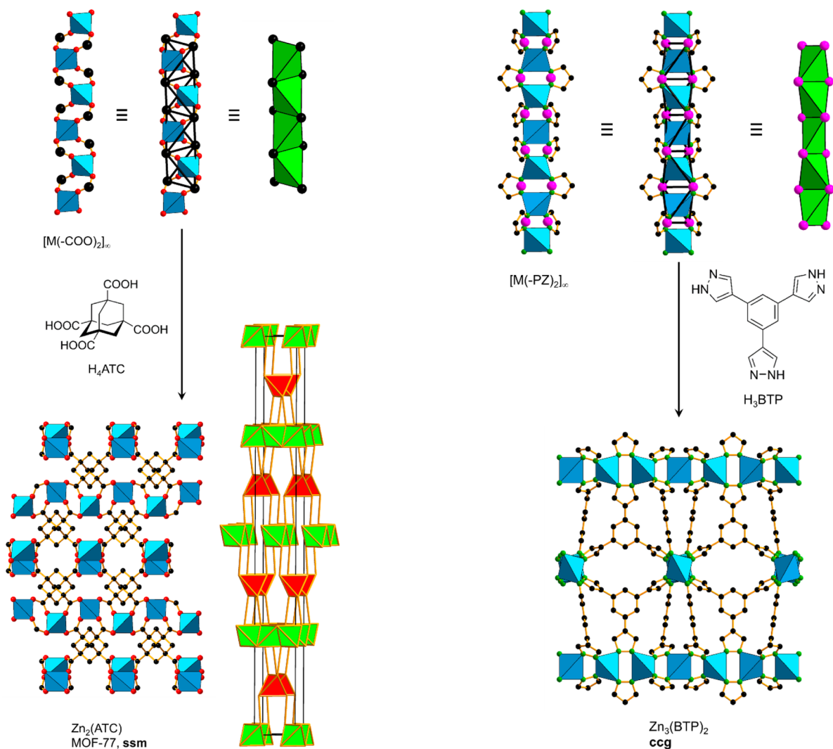
Figure 28. Crystal structure of MOF-77 and the underlying ssm net. The opposite edge-sharing tetrahedra rod SBUs are running in two directions. 6 Color code: black, C; red, O; blue polyhedra, metal.
