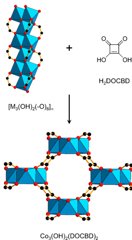
Figure 59. SBU and crystal structure of Co_3(OH)_2(DOCBD)_2 . The deconstruction in this particular case is not obvious. 226 Color code: black, C; red, O; blue polyhedra, metal.
