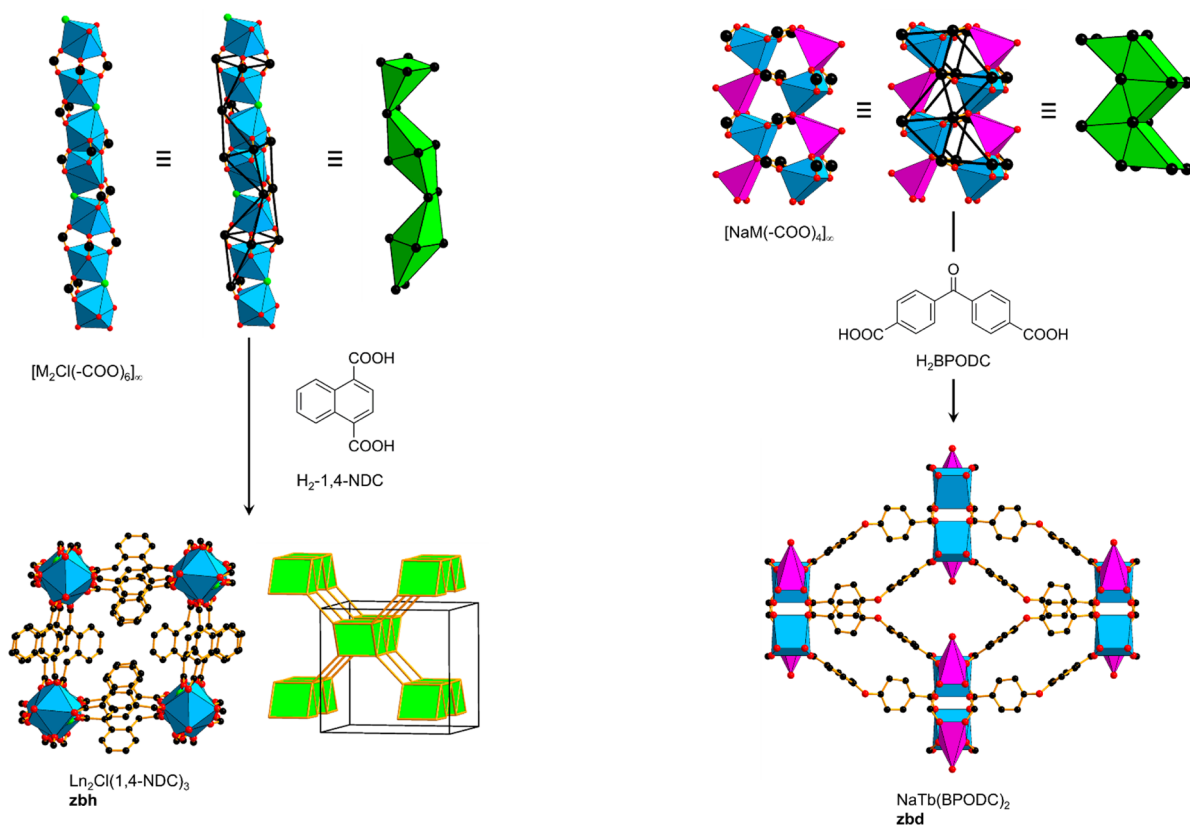
Figure 43. Linking of face- and edge-sharing trigonal prisms with ditopic linkers, leading to an anionic framework with zbh topology. 193 Color code: black, C; red, O; green, Cl; blue polyhedra, metal.
