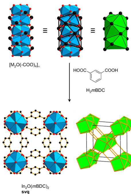
Figure 56. Linking of face-sharing tetragonal antiprism SBUs with angular, ditopic mBDC to produce In_2O(mBDC)_2 showing an underlying uninodal svq net. 218 Color code: black, C; red, O; blue polyhedra, metal.
