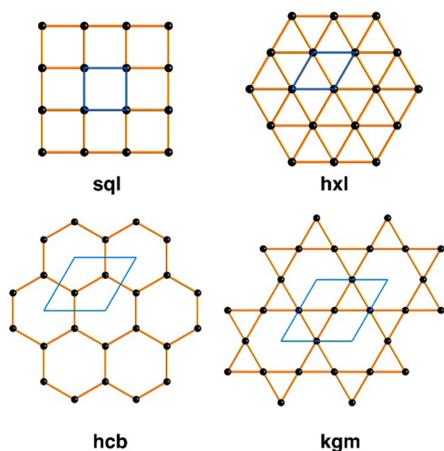
Figure 6. Invariant 2-periodic patterns.
