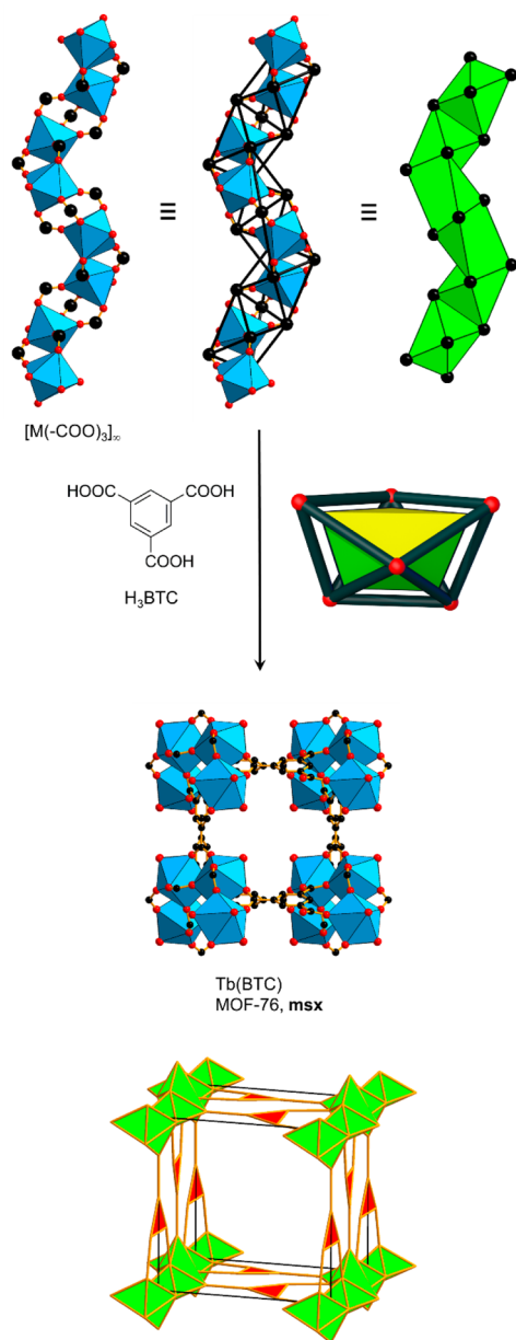
Figure 90. Single crystal structure of MOF-76 and its underlying 4-nodal (3,3,5,7)-c msx net. 6 The tiling of the diminished pentagonal bipyramid is highlighted. Color code: black, C; red, O; blue polyhedra, metal.
