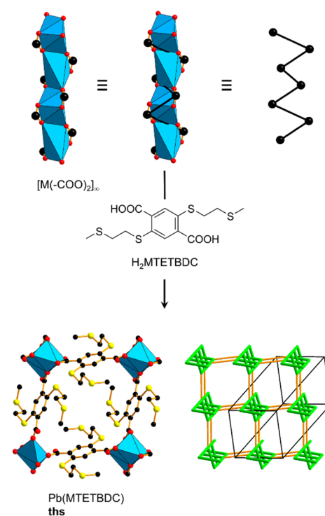
Figure 12. Single crystal structure of Pb(MTETBDC) . The 4-fold helices form an overall ths net. 96 Color code: black, C; red, O; yellow, S; blue polyhedra, metal.
