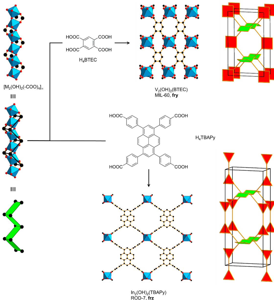
Figure 20. Zigzag ladder rod SBUs combined with tetrapotic linkers. Symmetric linkers lead to a binodal (3,4)-c fry topology, asymmetric linkers to a trinodal (3,4)-c frz topology. 129,134 Color code: black, C; red, O; blue polyhedra, metal.
