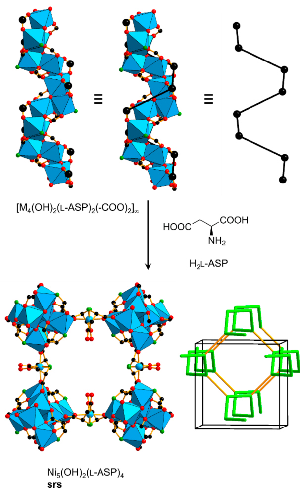
Figure 11. Rod of Ni_5(OH)_2(L-ASP)_4 consists of a chiral 4-fold helix that, when combined with a ditopic metallo-linker [Ni(L-ASP)_2]^{2-} , produces a 3-c srs topology net. 93 Color code: black, C; red, O; green, N; blue polyhedra, metal.
