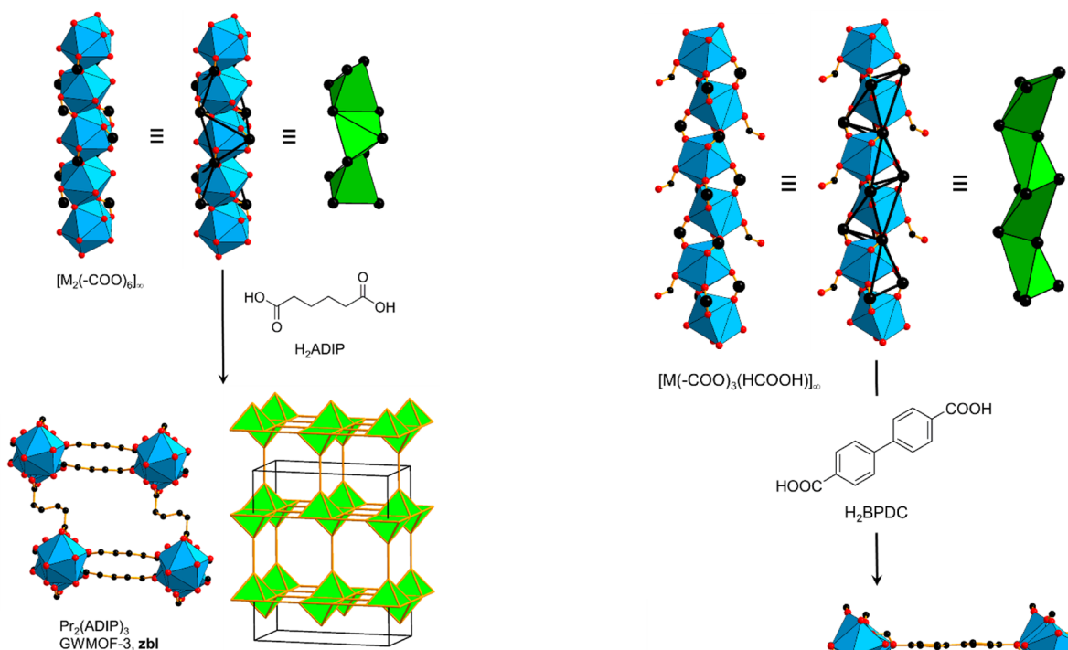
Figure 47. Linking of edge-sharing square pyramid SBUs with a flexible dicarboxylate. The resulting zbl net shows alternating layers of square pyramids that are interconnected. 186 Color code: black, C; red, O; blue polyhedra, metal.
