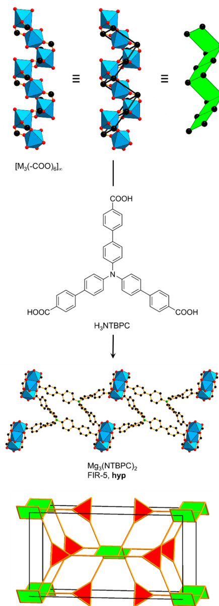
Figure 24. Single crystal X-ray structure of FIR-5 and the underlying (3,4)-c hyp net. 139 Color code: black, C; red, O; green, N; blue polyhedra, metal.
