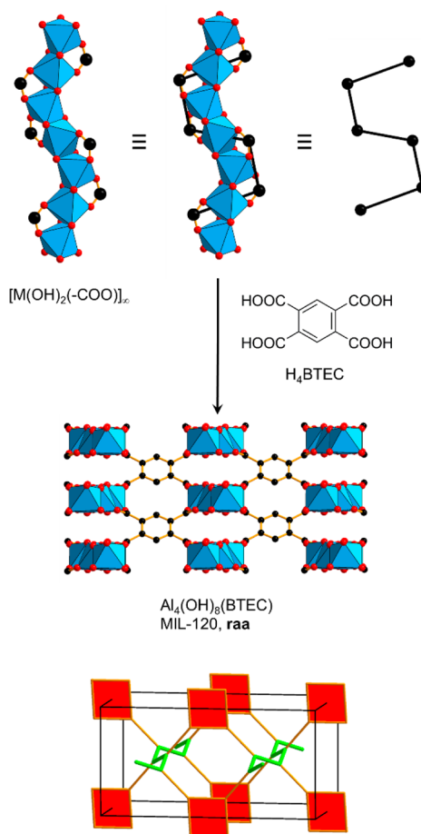
Figure 14. Single crystal structure of \text{Al}_4(\text{OH})_8(\text{BTEC}) , MIL-120. The helical rod SBUs are connected by tetratopic organic linkers yielding a (3,4)-c raa net. 100 Color code: black, C; red, O; blue polyhedra, metal.
