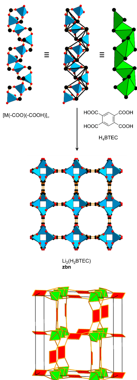
Figure 30. Combination of helical [M(-COO)(-COOH)]_{\infty} SBUs with tetratopic BTEC produces Li_2(H_2BTEC) . It is best described as a binodal (3,6)-c zbn net. 154 Color code: black, C; red, O; blue polyhedra, metal.
