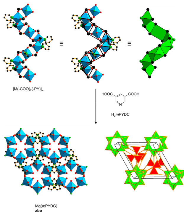
Figure 54. Linking of edge-sharing square pyramidal SBUs with bifunctional, tritopic \text{mPYDC} to produce \text{Mg}(\text{mPYDC}) , a chiral framework with 4-nodal \text{z pb} topology. 213,214 Color code: black, C; red, O; green, N; blue polyhedra, metal.
