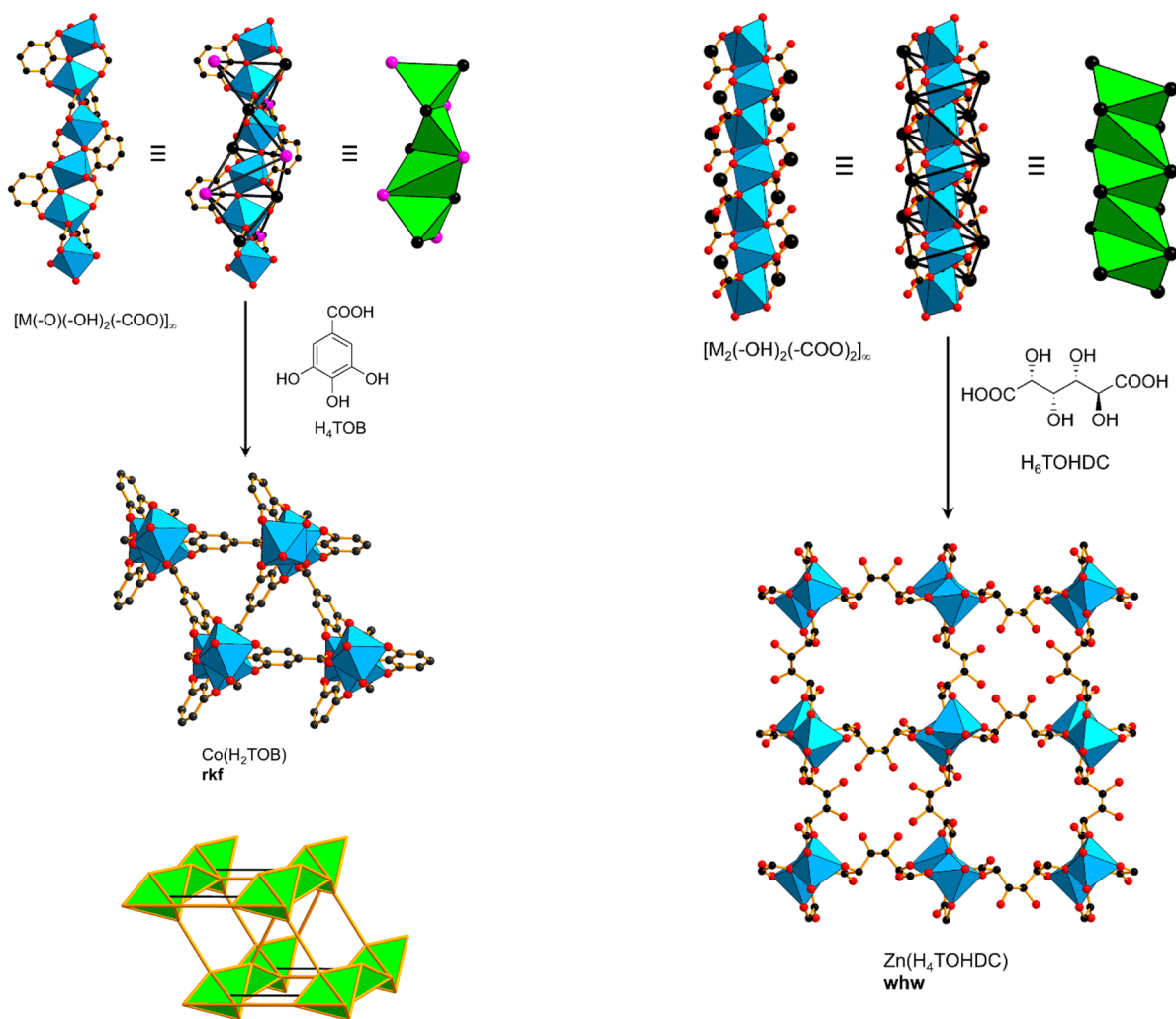
Figure 26. Combination of gallic acid with [M(-O)(-OH)_2(-COO)]_\infty SBUs leads to a family of chiral frameworks M(H_2TOB) with rkf topology. 152 Color code: black, C; red, O; blue polyhedra, metal; pink, points of extension.
