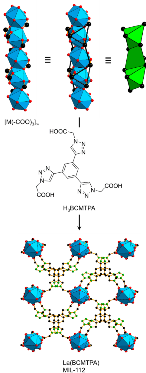
Figure 50. Flexible, tritopic linkers together with linked square pyramid SBUs produce MIL-112. 209 Color code: black, C; red, O; green, N; blue polyhedra, metal.
