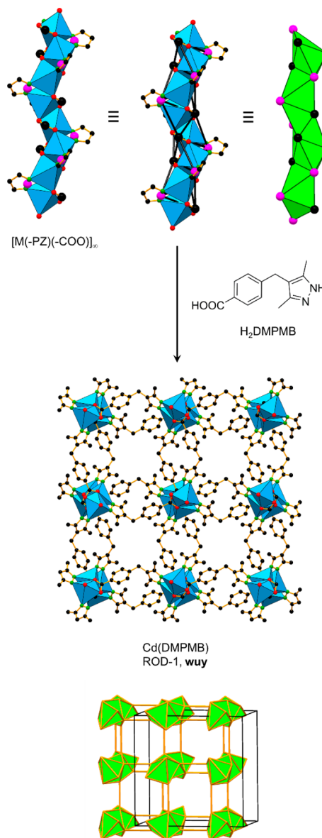
Figure 83. Single crystal structure of ROD-1. The flexible linker facilitates connections between the BC helices. The underlying topology is a uninodal 7-c wuy net. Color code: black, C; red, O; green, N; blue polyhedra, metal; pink, points of extension.
