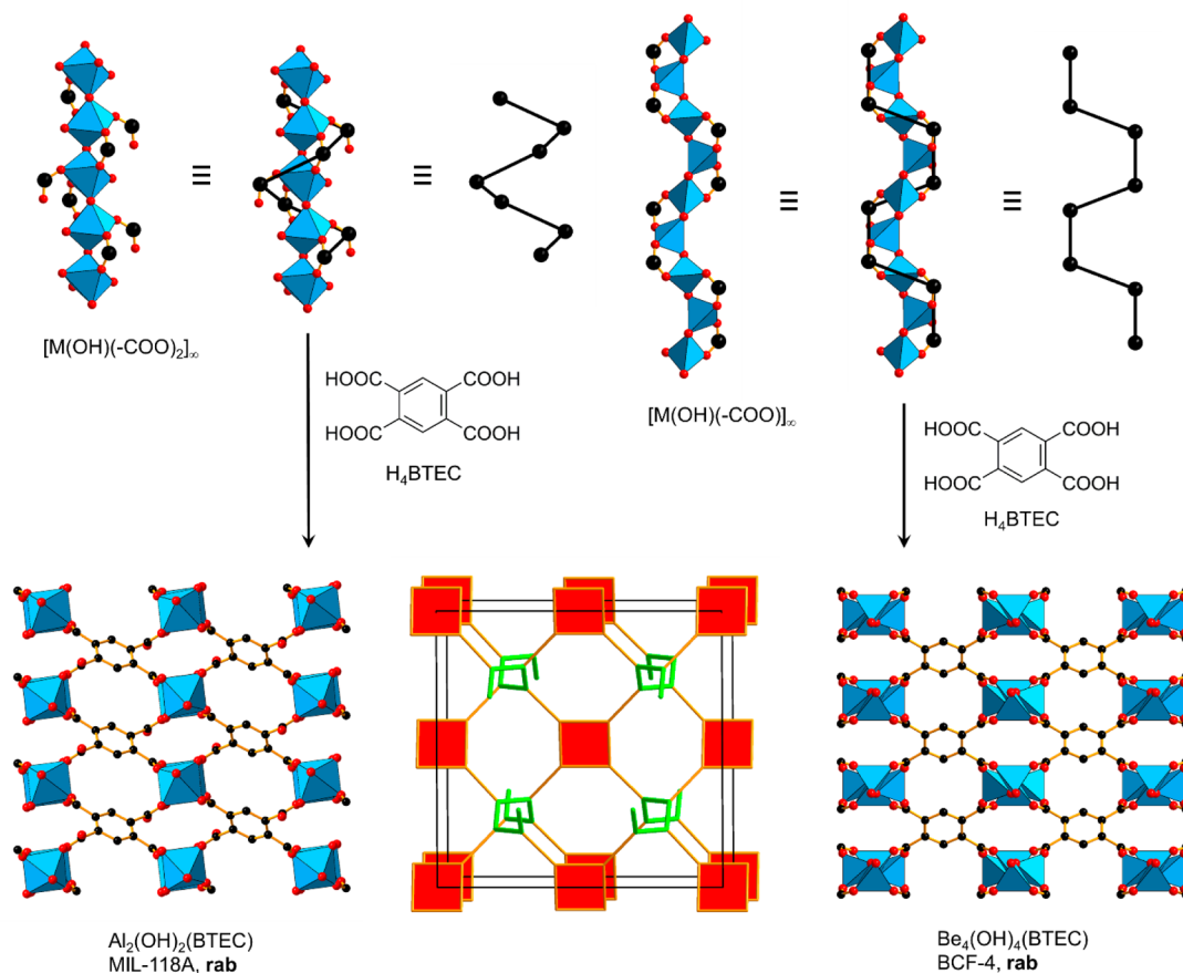
Figure 15. Two structurally different MOFs that show an underlying rab net topology. The 4-fold helices are connected through tetrapods. 101,102 Color code: black, C; red, O; blue polyhedra, metal.
