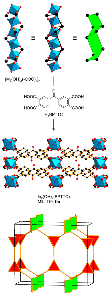
Figure 23. Single crystal structure of MIL-119 and its underlying frx net. 138 Color code: black, C; red, O; blue polyhedra, metal.
