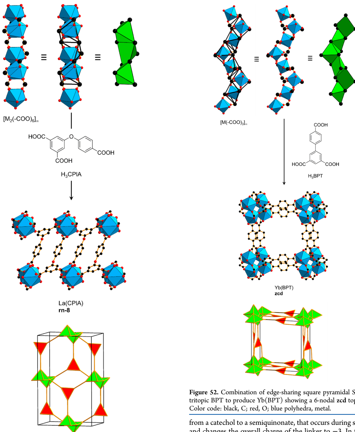
Figure 51. Flexible, asymmetric linker together with alternating, linked square pyramid SBUs produce La(CPIA). 210 Color code: black, C; red, O; blue polyhedra, metal.
