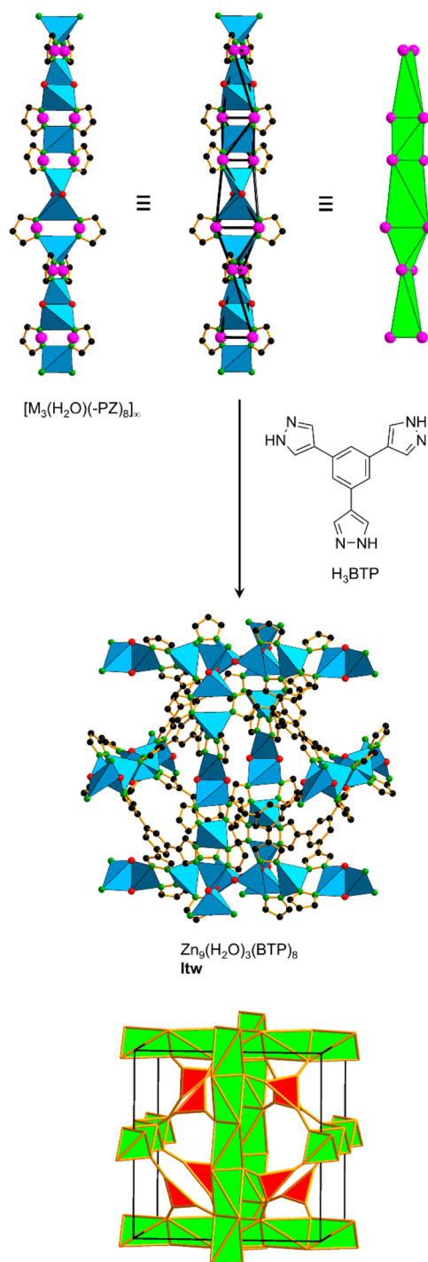
Figure 31. Idealized crystal structure of Zn_9(H_2O)_3(BTP)_8 , the only cubic 3-way pattern in rod MOFs. The underlying topology is a binodal (3,6)-c Itw net. 39 Color code: black, C; red, O; green, N; blue polyhedra, metal; pink, points of extension.
