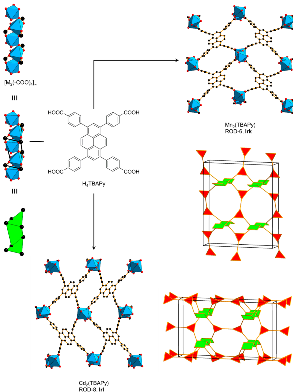
Figure 22. Single crystal structures of ROD-6 and ROD-8. ROD-6 crystallizes in the Irk topology, whereas ROD-8 shows positional disorder and is best described as an average between Irl (shown here) and Irk topology. 137 Color code: black, C; red, O; blue polyhedra, metal.
