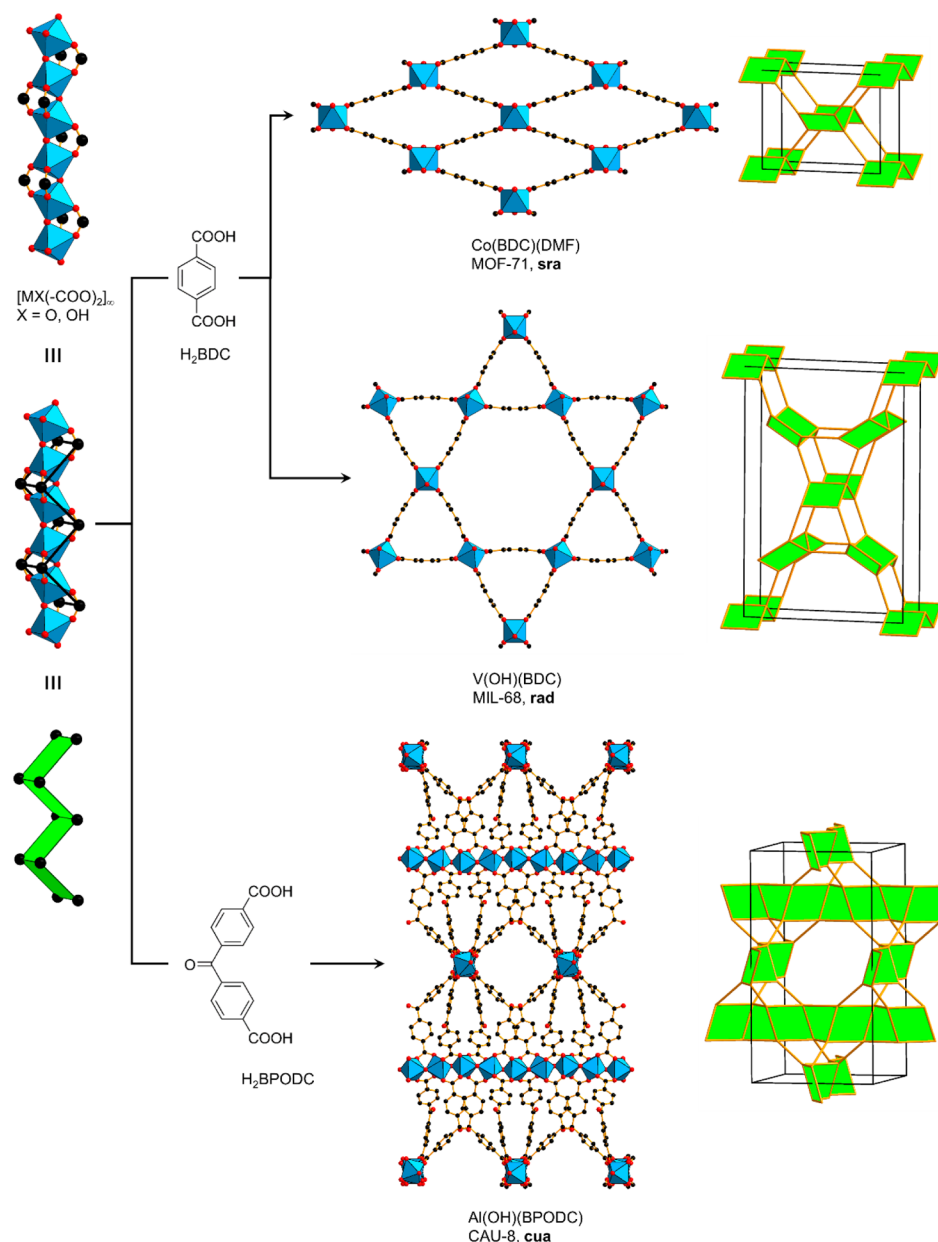
Figure 16. Three topologically different frameworks formed by zigzag ladders of general formula [MX(-COO)_2]_{\infty} ( X = O, OH ). Various angles subtended either at the SBU or the linkers facilitate different orientation of rod SBUs in 1-dimension ( sra , rad ) or in 2-dimensions ( cua ). 6,114,116 Color code: black, C; red, O; blue polyhedra, metal.
