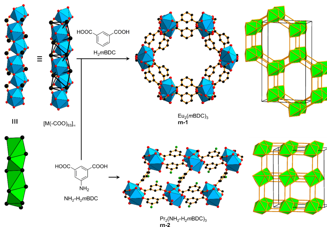
Figure 35. Linking of face-sharing octahedral SBU, [M(-COO)_3]_\infty , with angular dicarboxylates leading to different nets. 171,172 Color code: black, C; red, O; green, N; blue polyhedra, metal.
