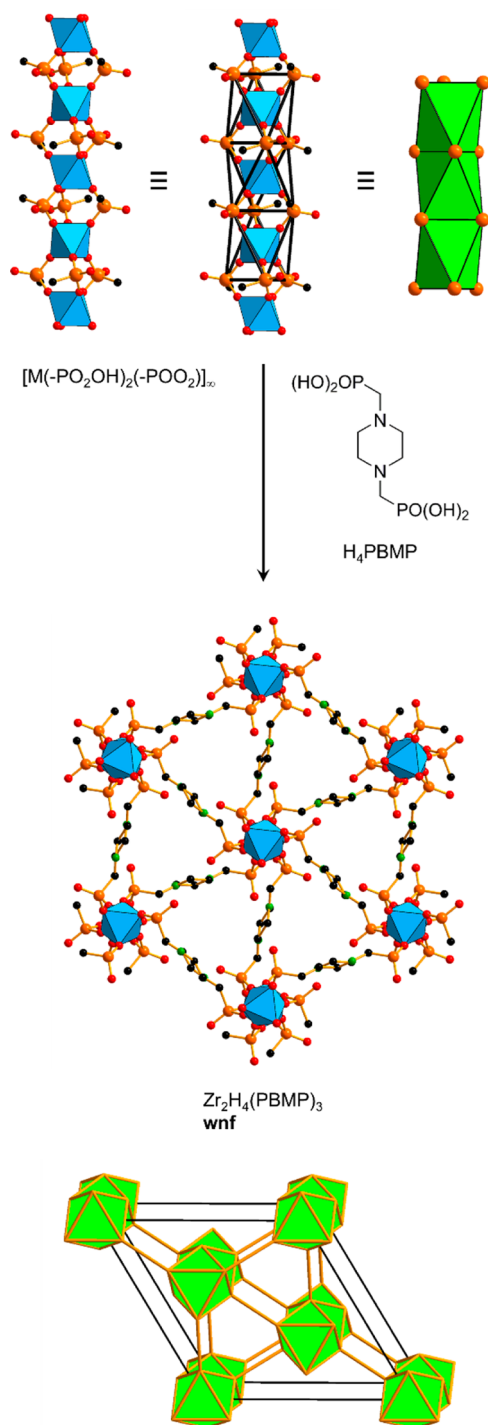
Figure 34. Crystal structure of Zr_2H_4(PBMP)_3 and its underlying uninodal 7-c net wnf . 169 Color code: black, C; red, O; green, N; orange, P; blue polyhedra, metal.
