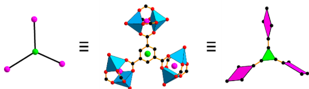
Figure 1. Center: the linker in HKUST-1 joined to three \text{Cu}_2(-\text{COO})_4 paddle wheel SBUs. 22 Left: the 3-c (green) and 4-c (magenta) nodes of the underlying net. Right: A fragment of the augmented net with nodes at the points of extension. Color code: black, C; red, O; blue polyhedra, metal.
