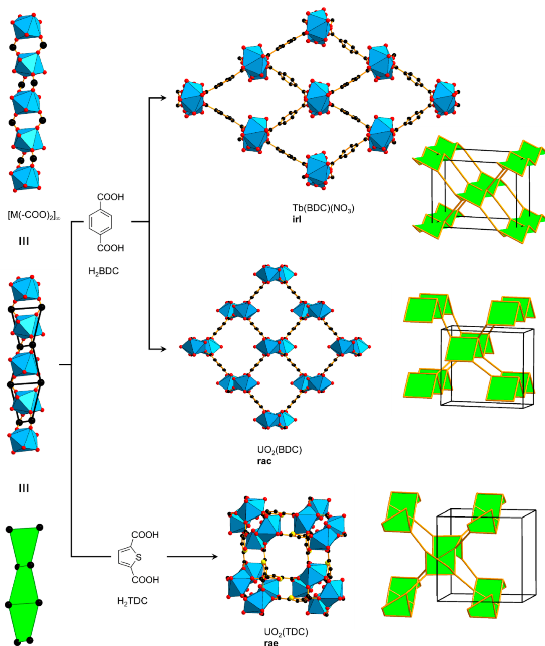
Figure 17. Single crystal structures and net topologies ( irl , rac , and rae ) of MOFs built from [M(-COO)_2]_\infty twisted zigzag ladder SBUs. 28,123 Color code: black, C; red, O; yellow, S; blue polyhedra, metal.
