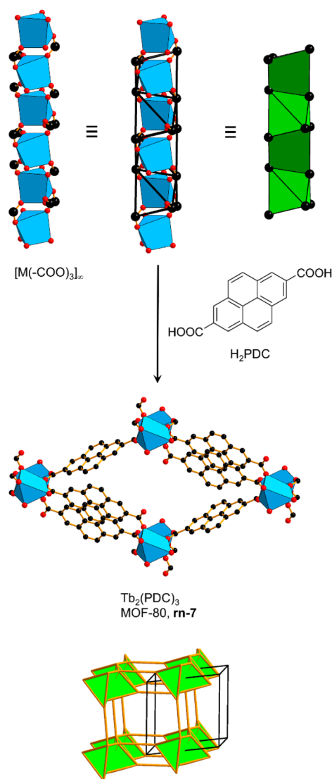
Figure 49. Combination of edge-sharing square pyramidal SBUs with a ditopic linker produce MOF-80 with a trinodal net topology. 6 Color code: black, C; red, O; blue polyhedra, metal.
