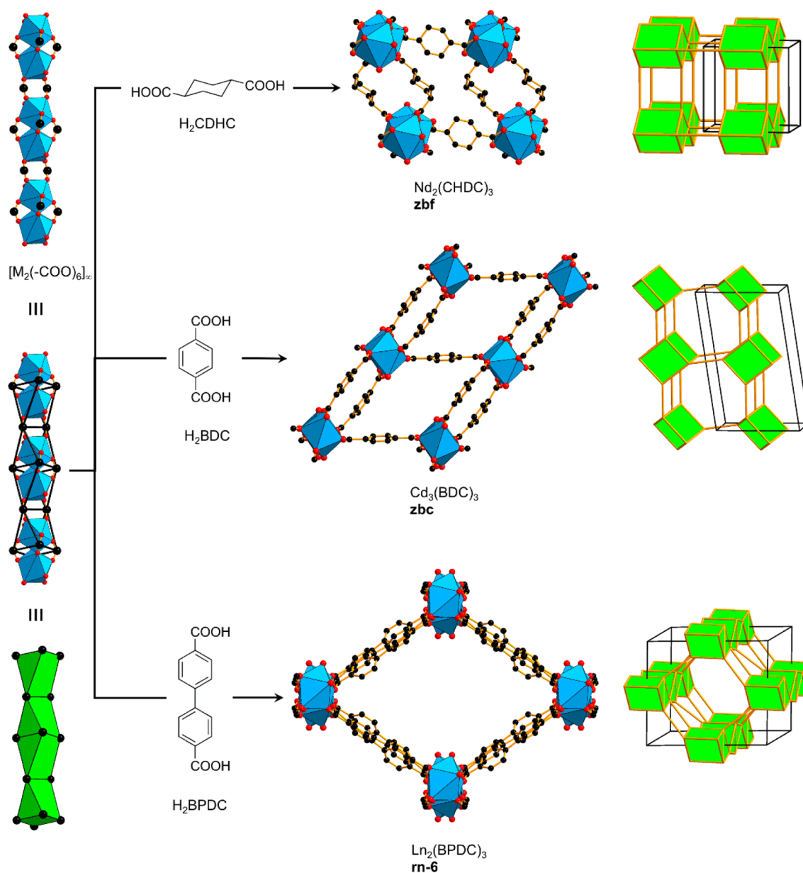
Figure 42. Linking of face- and edge-sharing trigonal prisms with ditopic linkers, leading to frameworks with zbf , 188 zbc , 189 and rn-6 topology. 190 Color code: black, C; red, O; blue polyhedra, metal.
