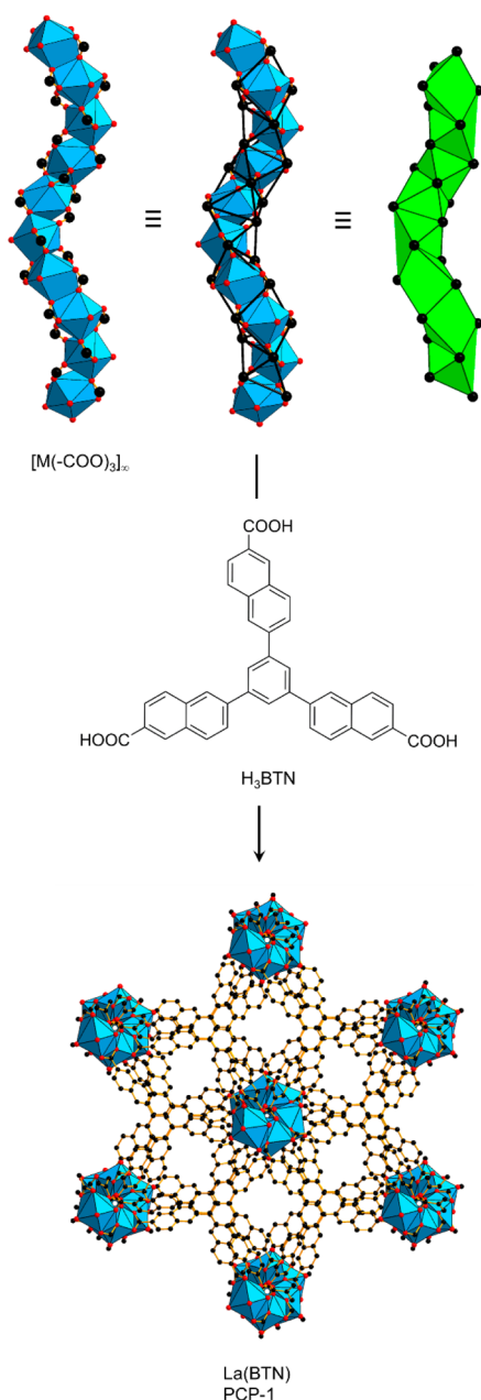
Figure 92. Crystal structure and rod SBU of La(BTN). 200 Color code: black, C; red, O; blue polyhedra, metal.
