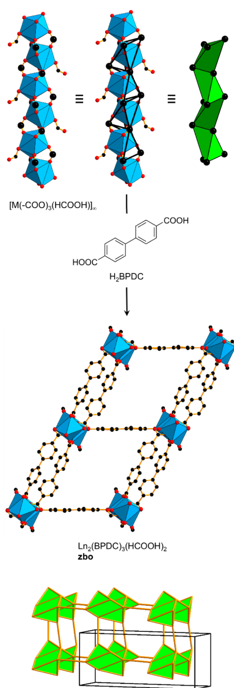
Figure 48. Joining of linked square pyramid SBUs into a framework with underlying zbo topology. 203 Color code: black, C; red, O; blue polyhedra, metal.
