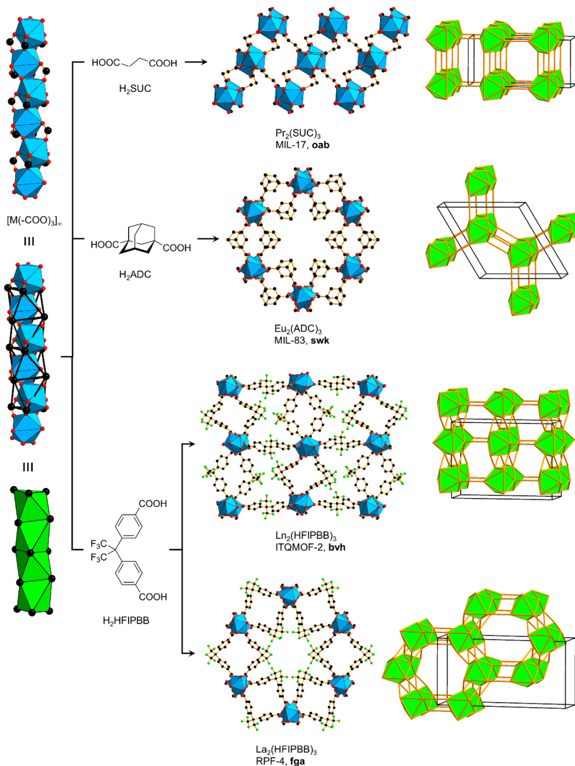
Figure 32. Linking of face-sharing octahedral SBUs, [M(-COO)_3]_\infty , with rigid and flexible dicarboxylates leads to a large structural diversity exemplified by oab, 155 swk, 160 bvh, 164 and fga nets, 165 respectively. Color code: black, C; red, O; green, F; blue polyhedra, metal.
