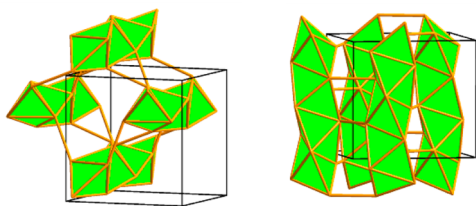
Figure 84. 7-c Net III with transitivity 1 6 and symmetry I4_122 . This is the unique minimal transitivity way to join BC helices, all of the same hand.
