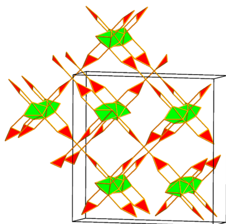
Figure 82. In the net hqx , the 3-c nodes are sufficiently widely spaced to allow a second copy of the structure with opposite hand to interpenetrate. The ideal symmetry of the pair of nets is I4_1/acd .
