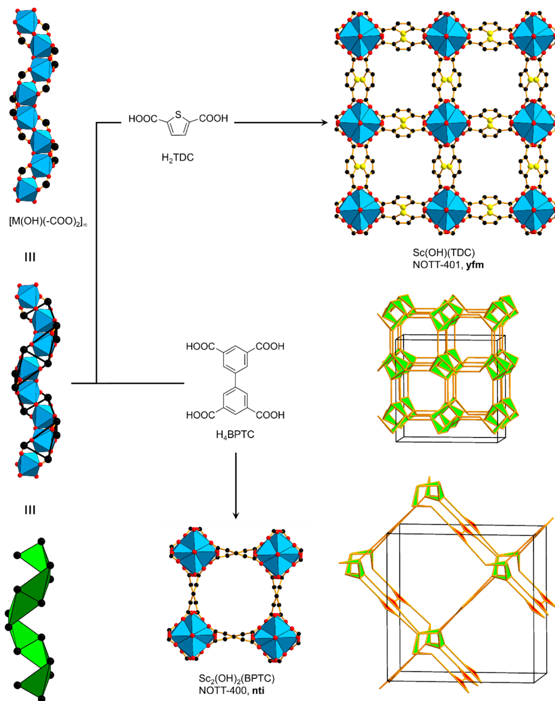
Figure 67. Structural diversity when linking [M(OH)(-COO)_2]_{\infty} helical ribbon SBUs with ditopic or tetratopic carboxylates. The resulting nets show either 5-c yfm or (3,5)-c nti topology. 232 Color code: black, C; red, O; yellow, S; blue polyhedra, metal.
