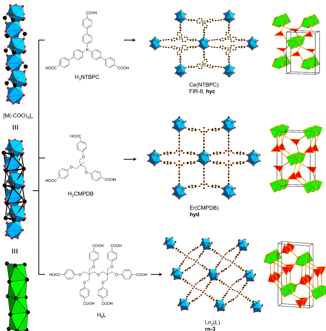
Figure 39. Linking of face-sharing octahedra with a tritopic linkers of different shape and a hexatopic linker leads to frameworks with hyc, 178 hyd, 179 and rn-3 topologies, 181 respectively. Color code: black, C; red, O; green, N; blue polyhedra, metal.
