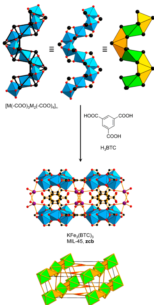
Figure 78. Crystal structures and net topology of MIL-45. The rod SBUs is formed by face-sharing octahedra and tetrahedra. 243 Color code: black, C; red, O; blue polyhedra, metal; purple, K.
