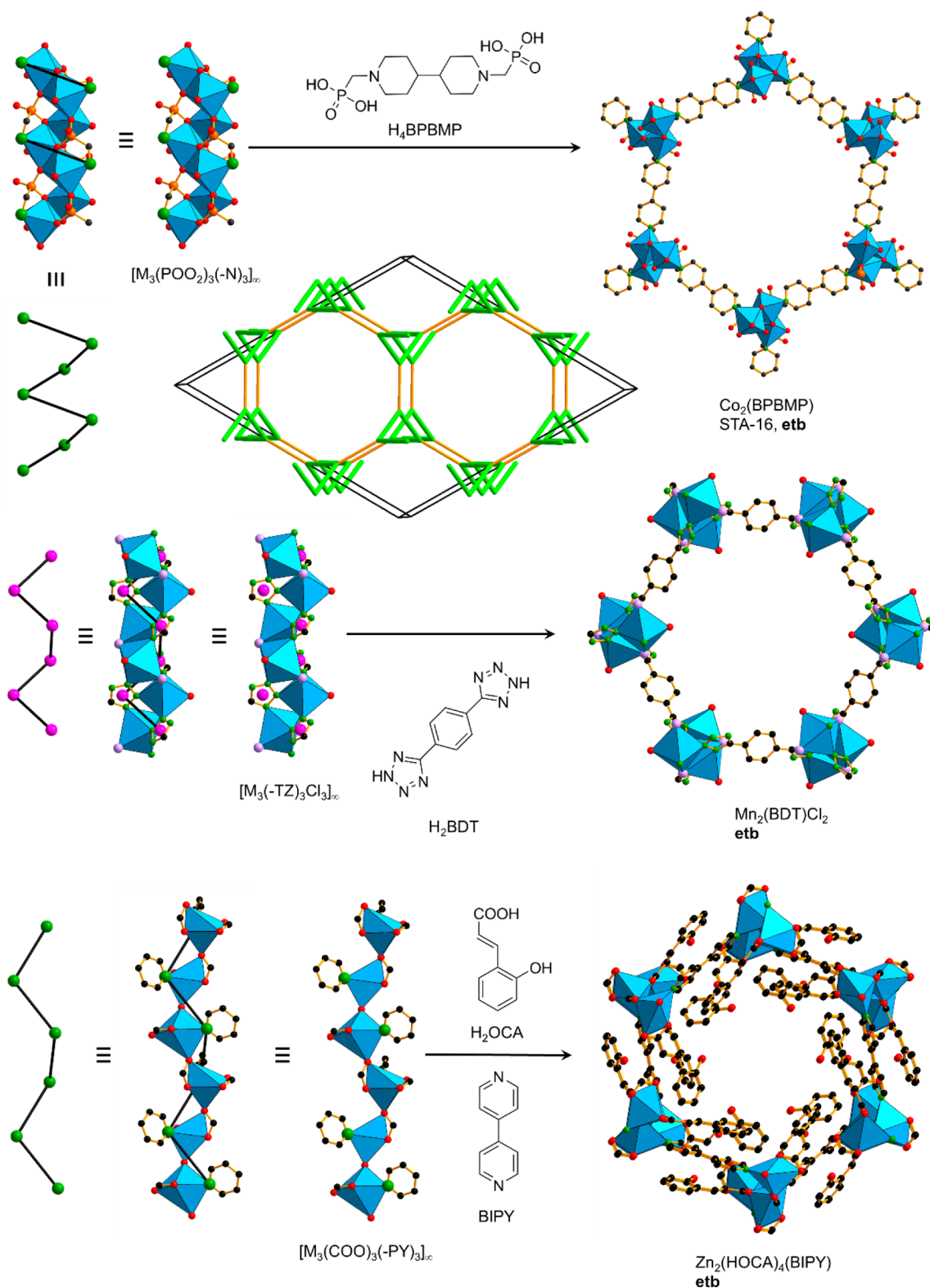
Figure 10. MOFs, showing etb topology, formed by rod, simple helical SBUs. Each node, marked as a large sphere, is 3-c, with 2 coordination within the trifold helix and one to the linker. 88–90 Color code: black, C; red, O; green, N; orange, P; lavender, Cl; blue polyhedra, metal; pink, points of extension.
