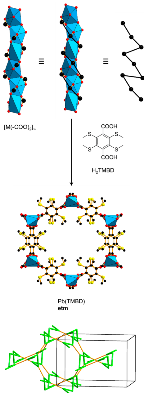
Figure 13. Single crystal structure of \text{Pb}(\text{TMBD}) that shows an underlying etm topology net. 97 Color code: black, C; red, O; yellow, S; blue polyhedra, metal.
