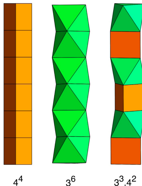
Figure 8. Examples of rods that are cylinder tilings.
