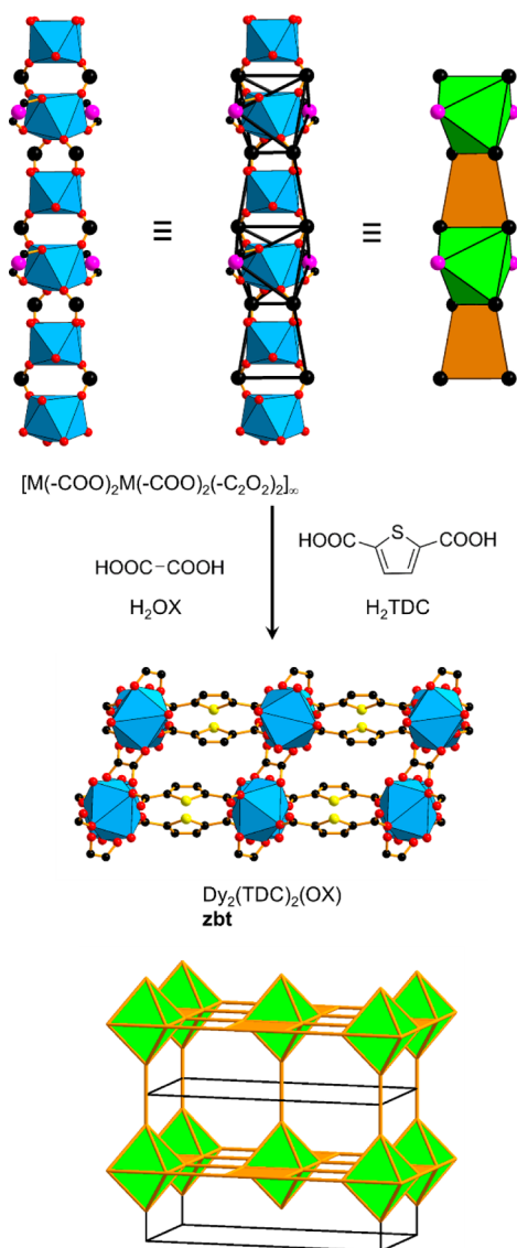
Figure 61. Crystal structure of \text{Dy}_2(\text{TDC})_2(\text{OX}) and the underlying zbt net. 228 Color code: black, C; red, O; blue polyhedra, metal; pink, points of extension.
