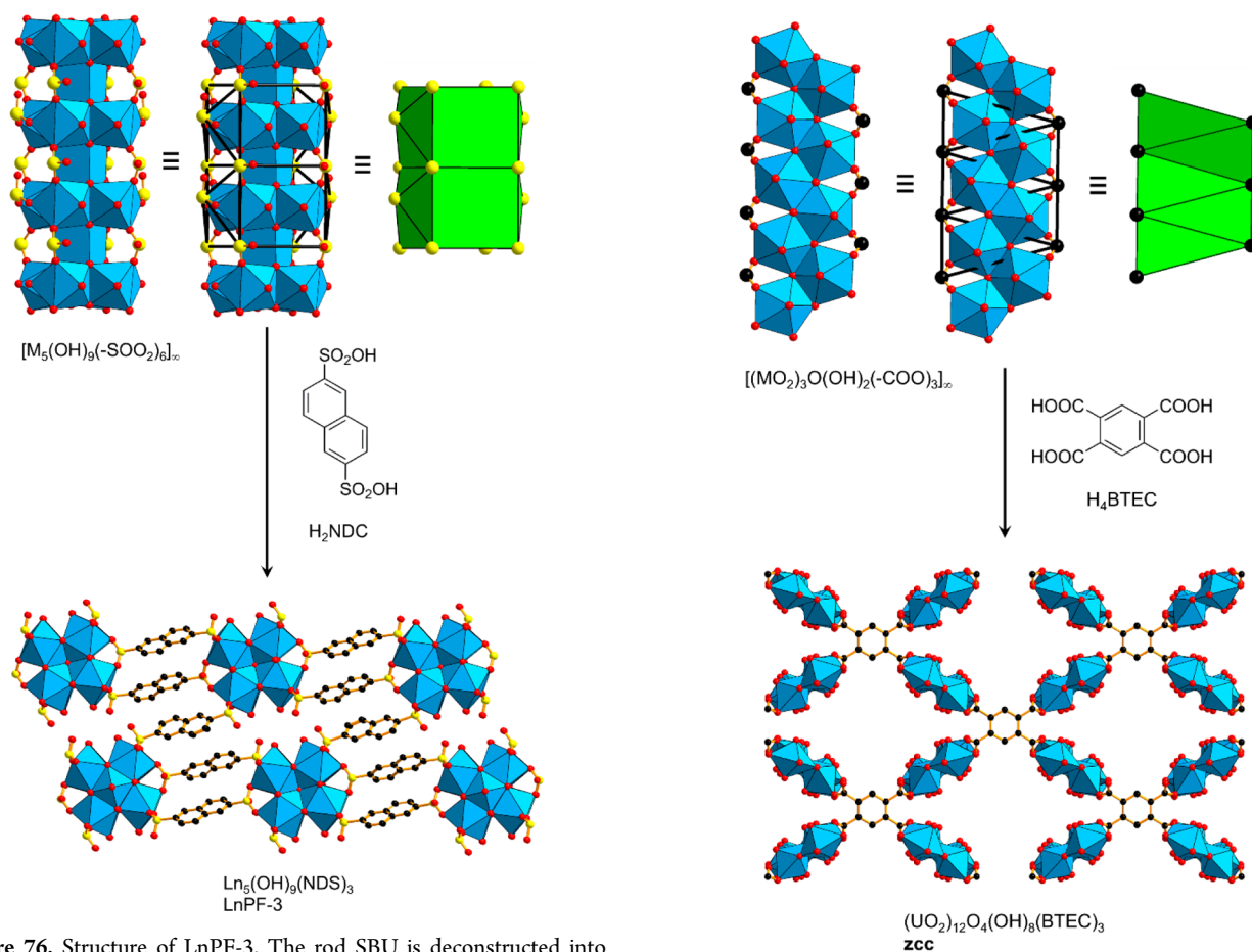
Figure 76. Structure of LnPF-3. The rod SBU is deconstructed into linked bicapped tetragonal prisms. 221 Color code: black, C; red, O; yellow, S; blue polyhedra, metal.
