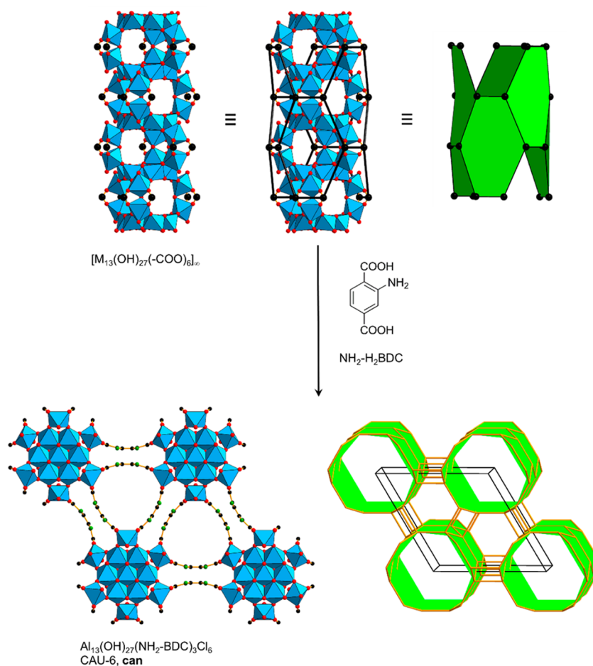
Figure 80. Linking of column-shaped SBUs with linear linkers to produce CAU-6, \text{Al}_{13}(\text{OH})_{27}(\text{NH}_2\text{-BDC})_3\text{Cl}_6 . It crystallizes as a zeolitic 4-c can net. 245 Color code: black, C; red, O; green, N; blue polyhedra, metal.
