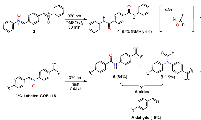
Scheme 2. Photoinduced rearrangement reactions of model compound 3 (1) and ^{13}C -labeled COF-115 (2).
