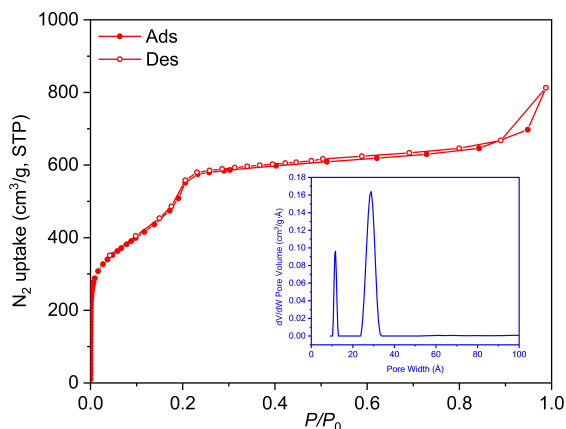
Figure 2. N_2 sorption isotherm of COF-115 at 77 K and its pore size distribution profile (inset).
