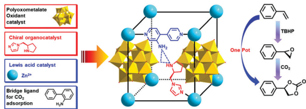
Fig. 13 (left) Synthetic procedure used to form a polyoxometalate-based MOF highlighting the materials' constituents, including the polyoxometalate oxidant catalyst (gold polyhedra), chiral organocatalyst, Lewis acid catalyst ( \text{Zn}^{2+} , cyan ball), and bridging ligand used to adsorb \text{CO}_2 . The organic linkers ( \text{NH}_2 -bipyridine) in the MOF are represented as black lines. (right) One pot asymmetric cyclic carbonate formation from the olefin and \text{CO}_2 achieved by tandem catalysis.
